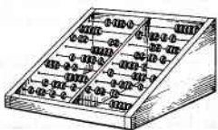
abace (1)
